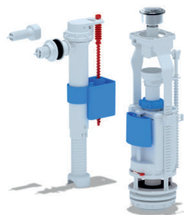
Fill and flush set, plastic side fitting
