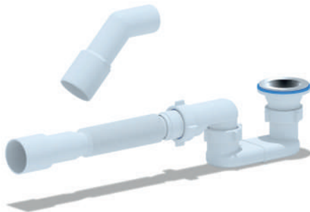
Flat trap for shower tray, two pipes
