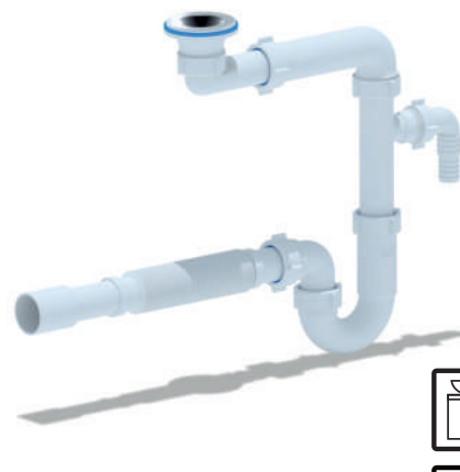
Trap with waste, flexible pipe
